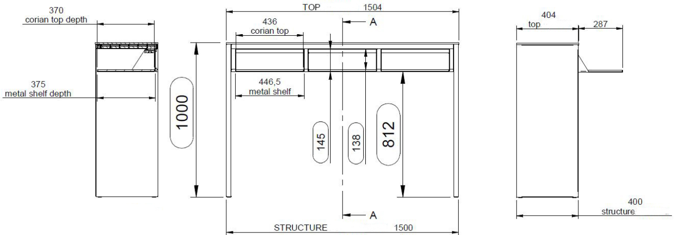
Figure 2 – XO WORKTOP – dimensions (mm)
